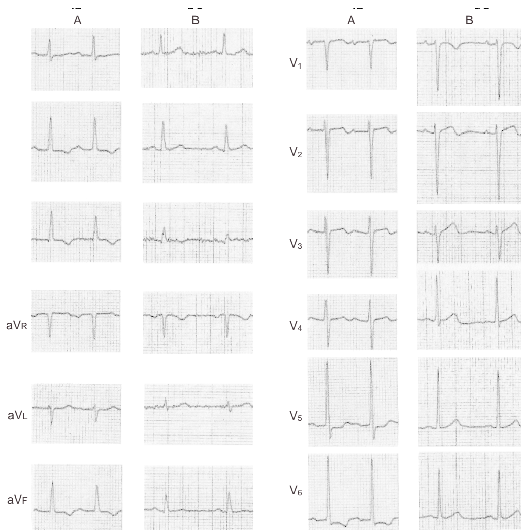
Fig. 3 Twelve-lead electrocardiograms
